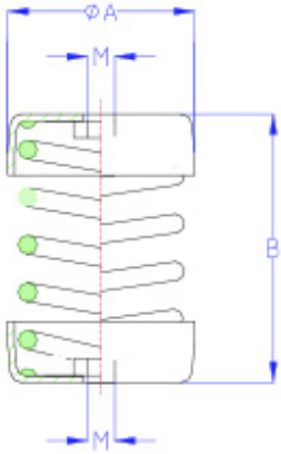
MLC-INOX
