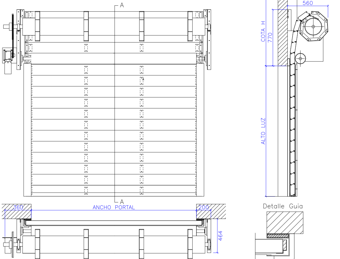
ENROLLABLE CORTAFUEGO Ei60
