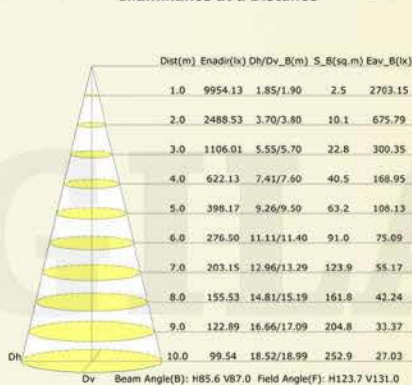
Illuminance at a Distance
