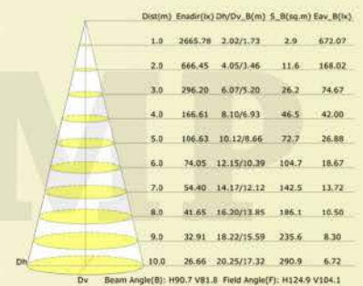
Iluminance at a Distance
