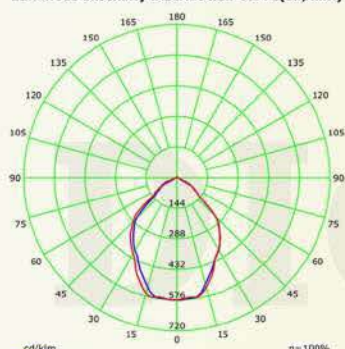
Luminous Intensity Distribution Curve(cd/klm)
