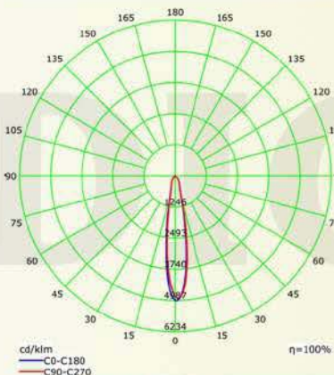
Luminous Intensity Distribution Curve(cd/klm)
