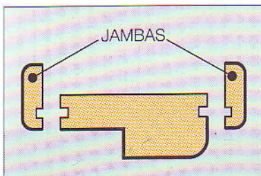
Ref. 7 Batidero con jambas
