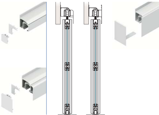
1 puerta - carril individual a pared 1 door - single track to wall
