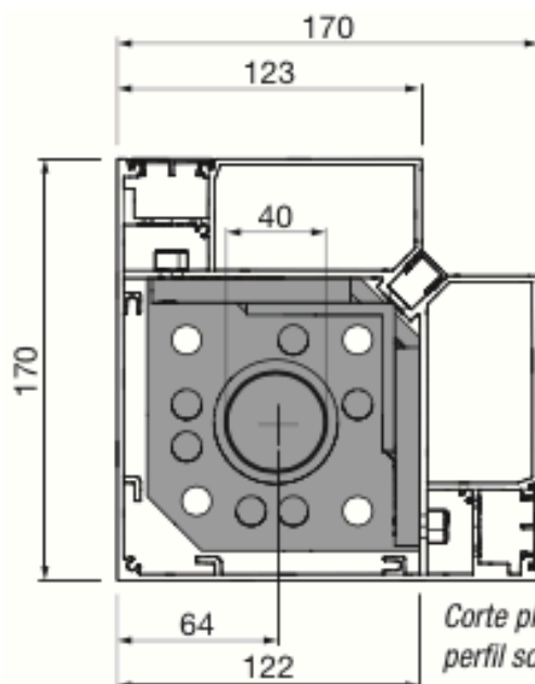
Foot plate / corner support profile section
