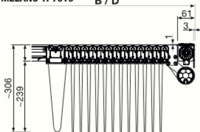
Side view / Vista lateral
