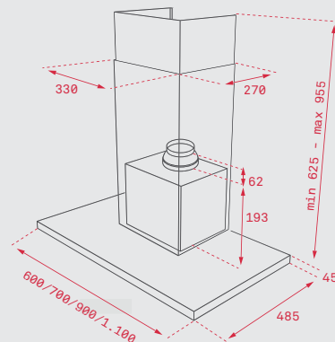
DLH 686 T/786 T/986 T/1186T
