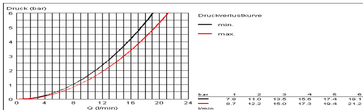
13928-13929 (Normal)
