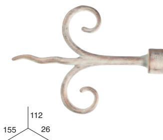
TERMINAL "LIS"
