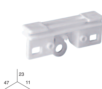
CORREDERA MAESTRA
